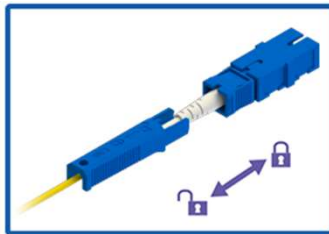
② Insert matching tool
